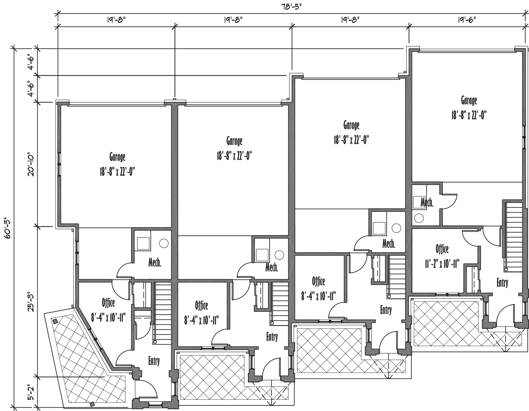
CASA ROMANA BUILDING ONE - FIRST FLOOR PLAN
